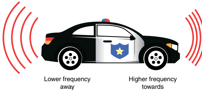
Figure 7.4 Doppler effect
