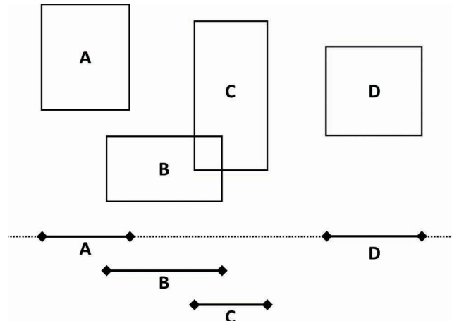
Figure 10.13 AABB intervals along the x -axis
