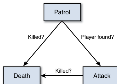
Figure 4.1 Basic stealth AI state machine
