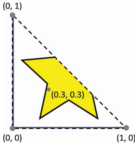
Figure 5.9 Texture mapping applied to a triangle
